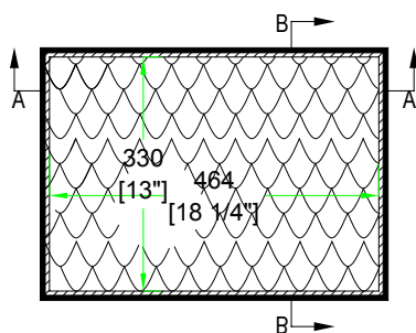
TOP VIEW OF COVER
