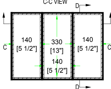
TOP VIEW OF BASE
