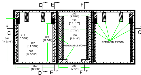
TOP VIEW OF BASE
