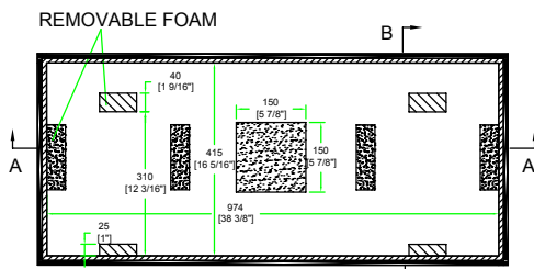
TOP VIEW OF COVER
