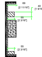
B-B VIEW
